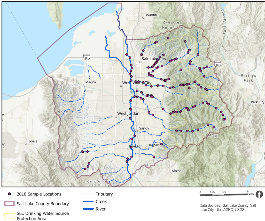
Figure 13. 2018 Field Parameter Sampling Locations
