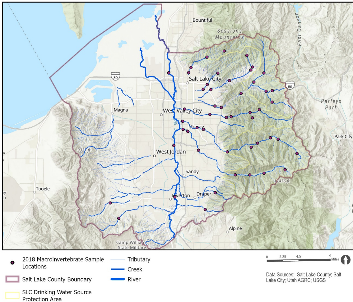
Figure 15. 2018 Macroinvertebrate Sampling Locations
