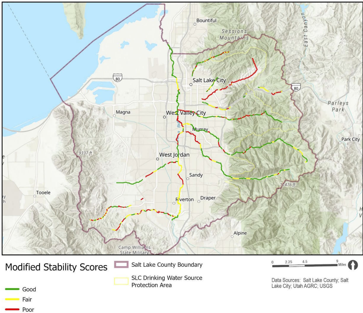
Figure 16. Stream Channel Stability Analysis
