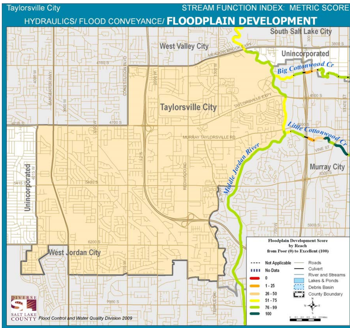
Figure 11. Hydraulics Function—Floodplain Development in Taylorsville City
