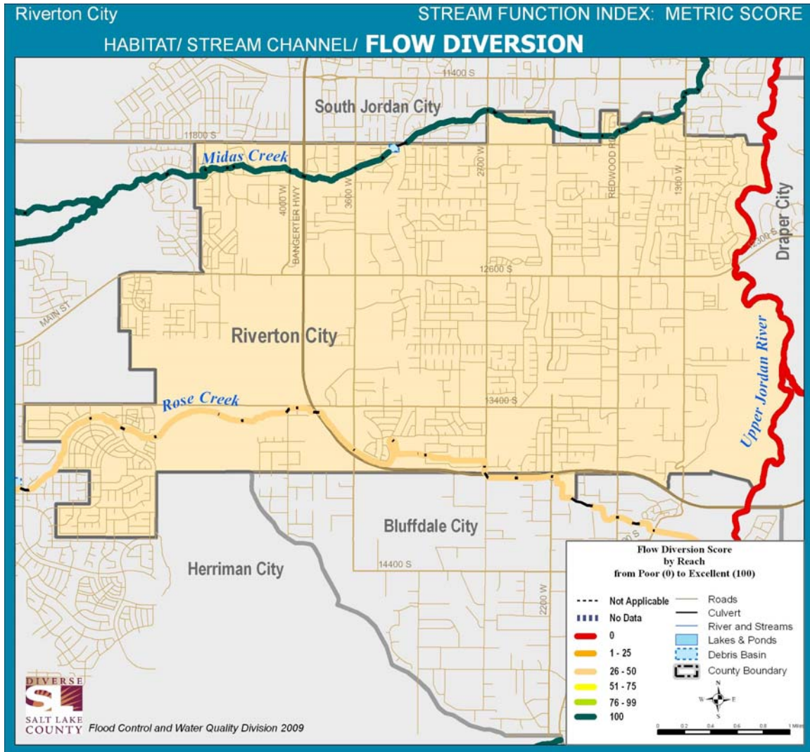
Figure 7. Habitat Function—Flow Diversion in Riverton City
