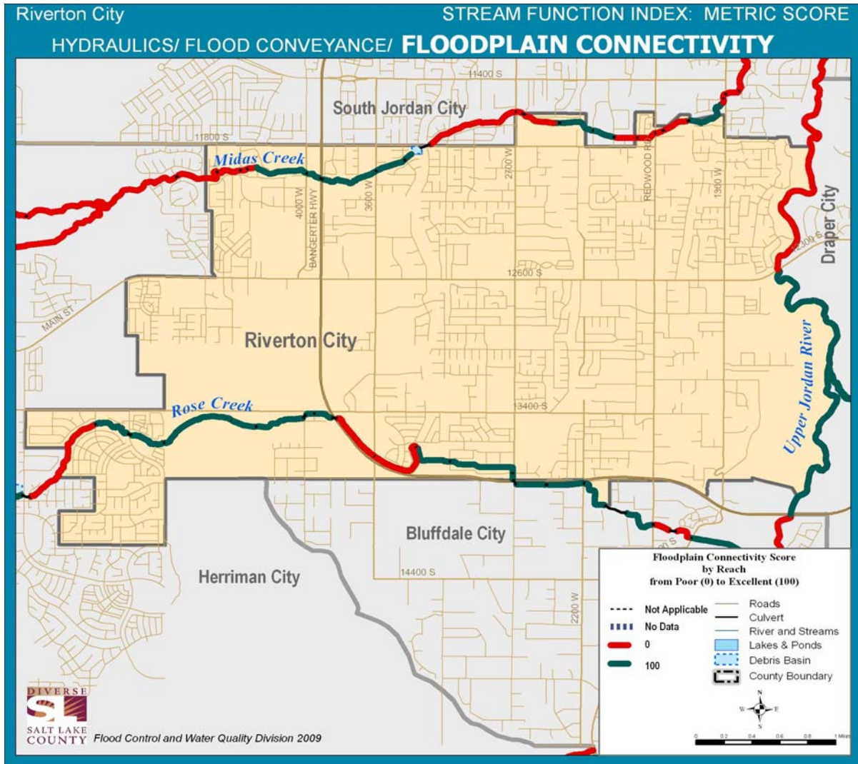
Figure 12. Hydraulics Function—Floodplain Connectivity in Riverton City
